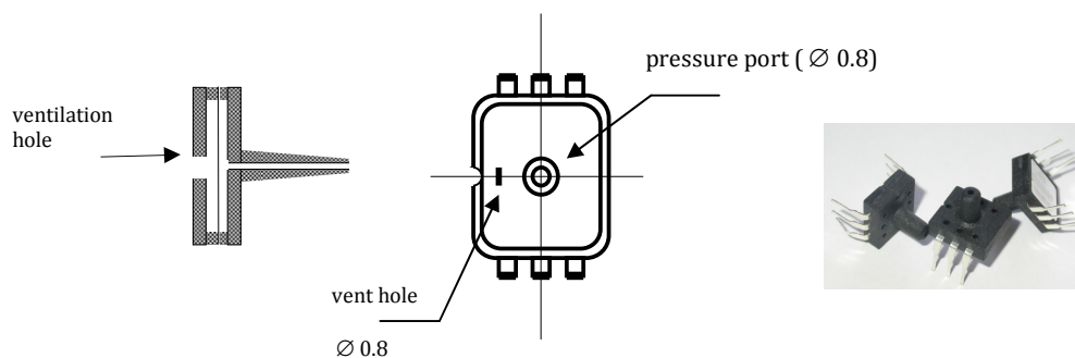
Fig. 2, principle of a gauge type pressure sensor
