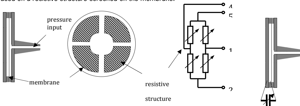
Fig1a. Principle of a pressure sensor strain gauge resistor
