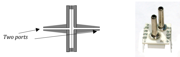
Fig 4, Principle of differential pressure sensor.
